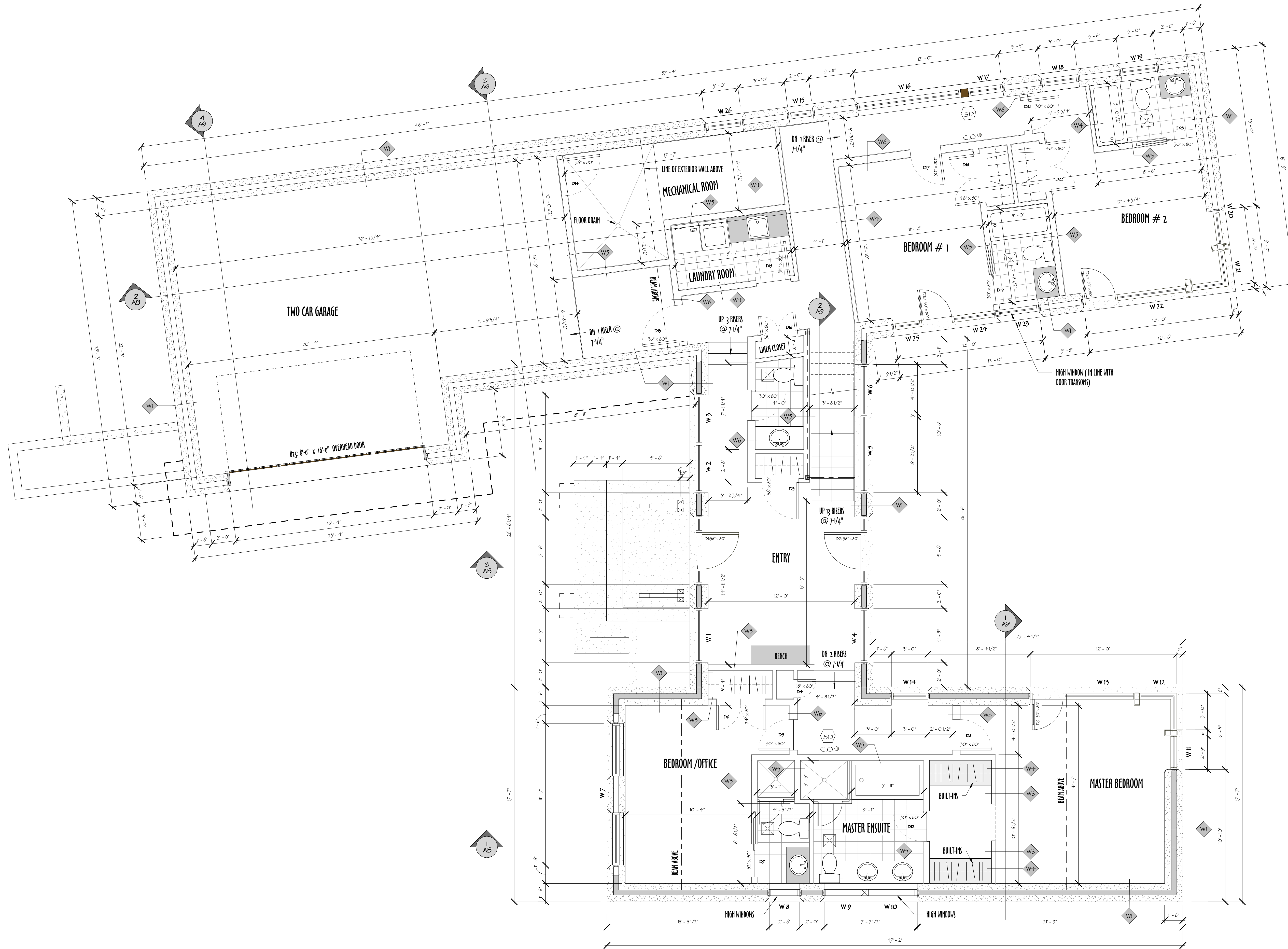
1 MAIN FLOOR PLAN A3 1/4" = 1'-0"
