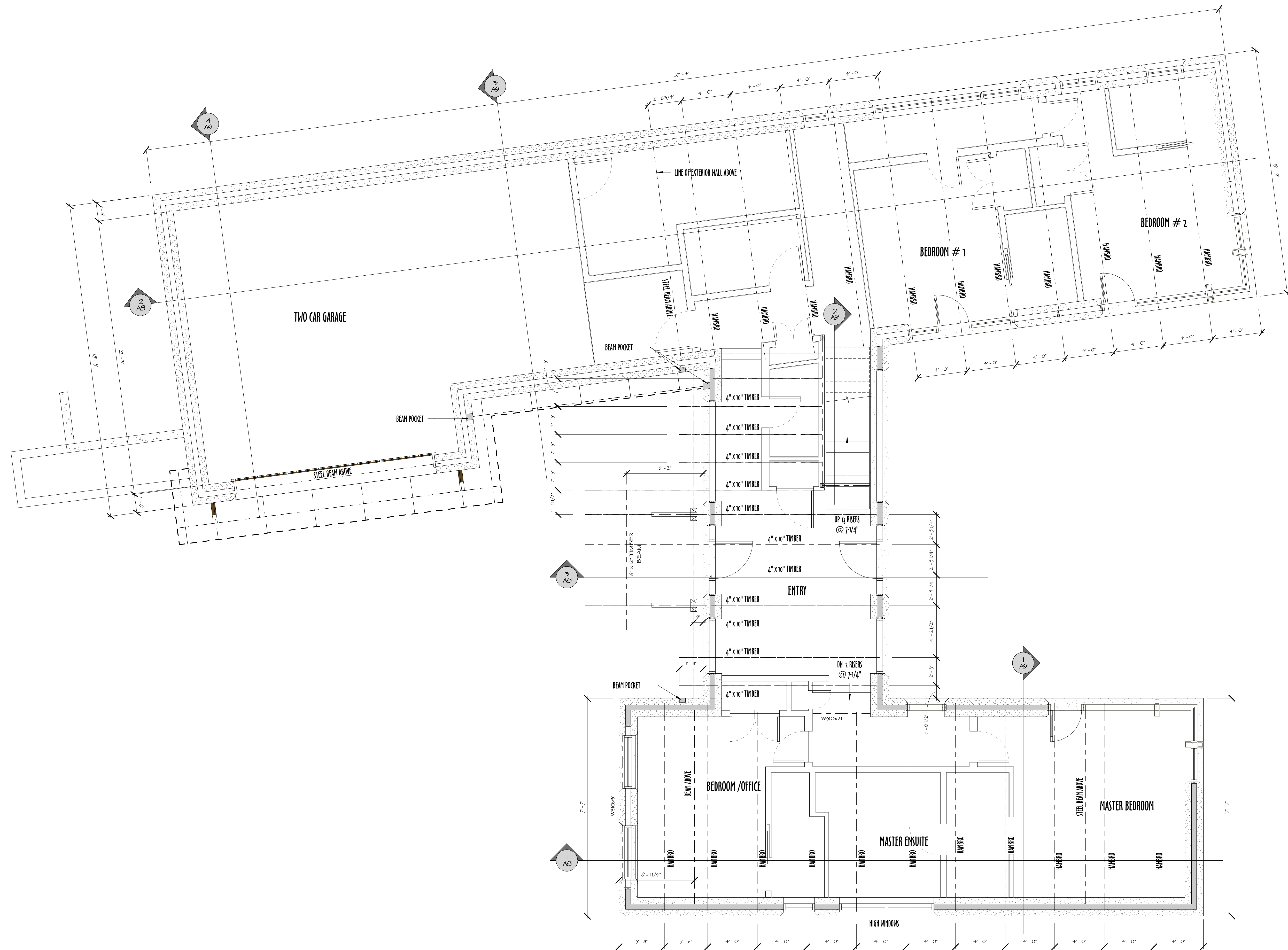
1 MAIN FLR - STRUCTURE A3.1 1/4" = 1'-0"
