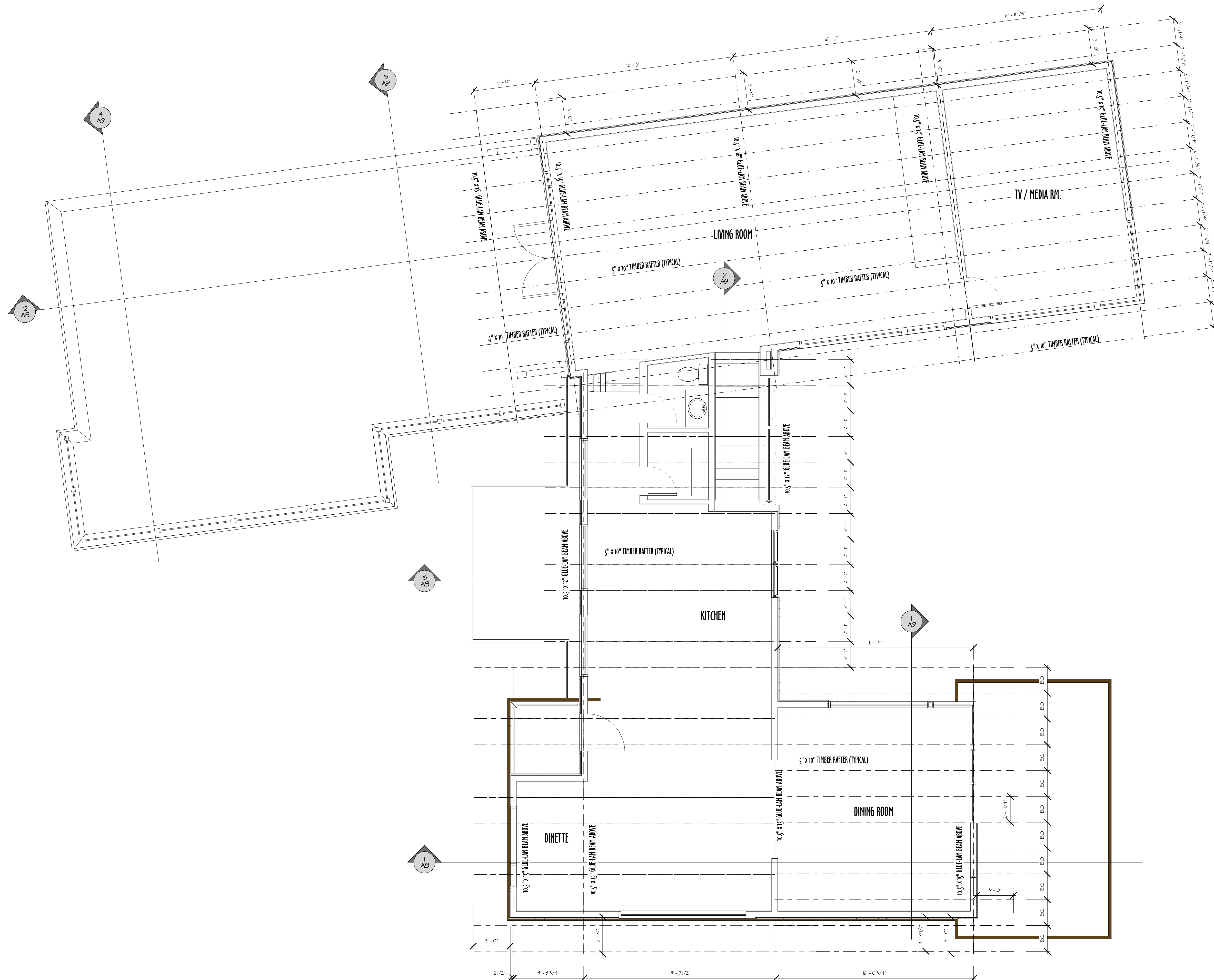
1 UPPER FLR - STRUCTURE A4.1 1/4" = 1'-0"
