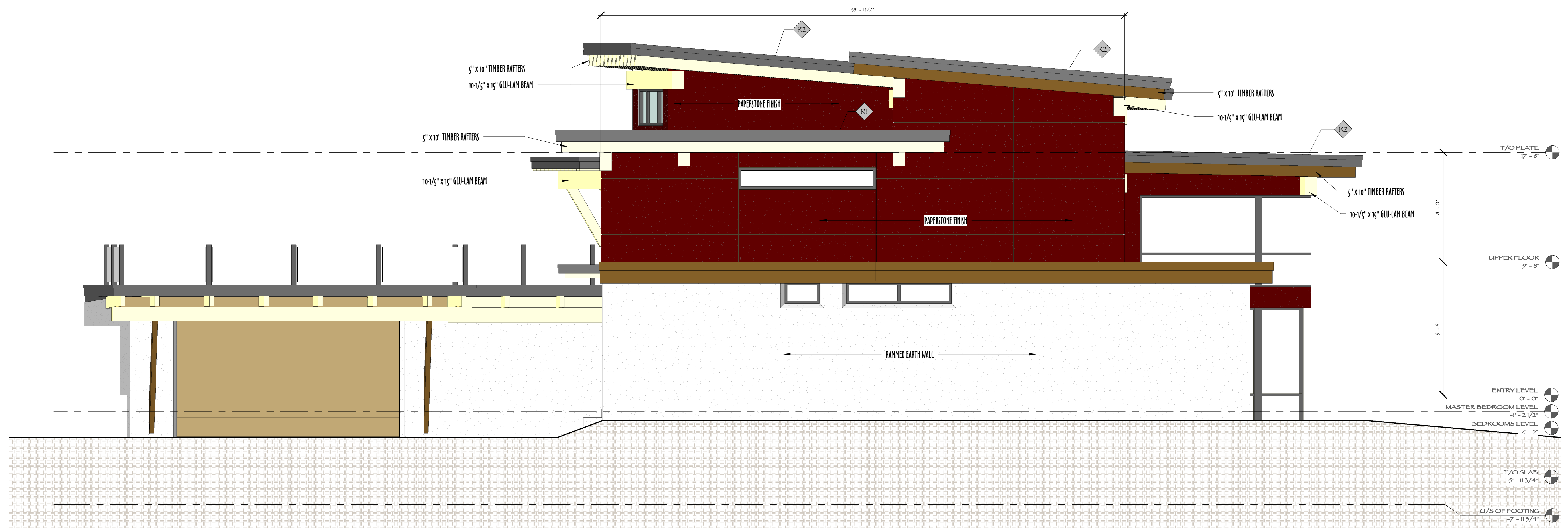
1 EAST ELEVATION 1/4" = 1'-0"
